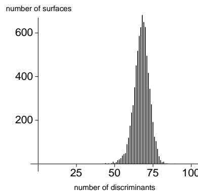
Figure 1: Number of distinct discriminants at primes with reduction to rank 18
